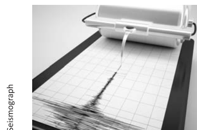
Earthquake, Santiago, Chile, 27 October 2010
